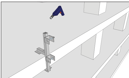
Easily adjusted with impact drill
